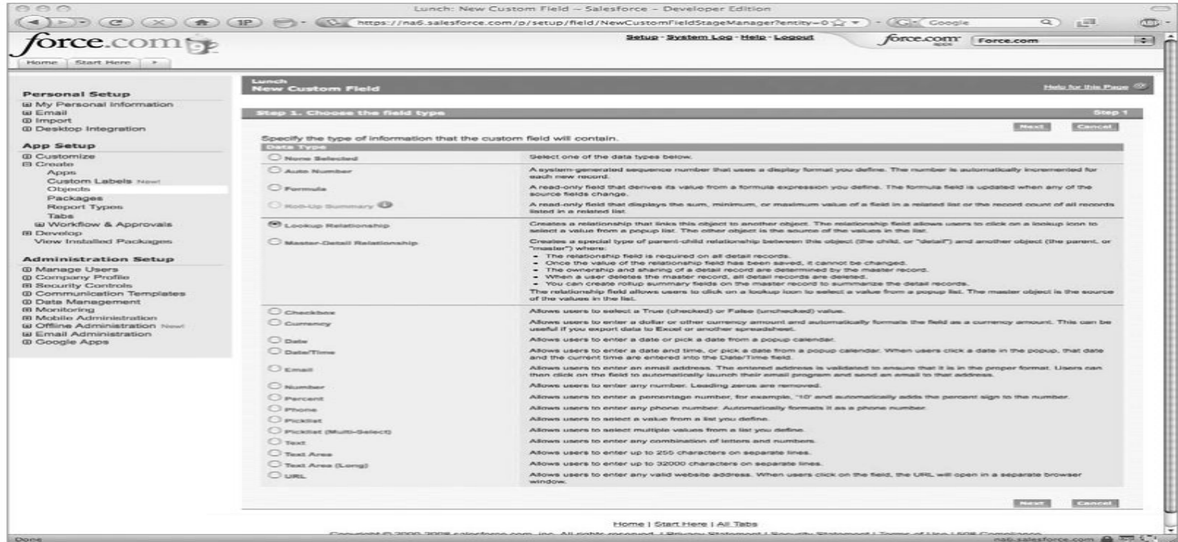
FIGURE 11-10 Selecting the Lookup Relationship data type allows you to link data for two objects.
